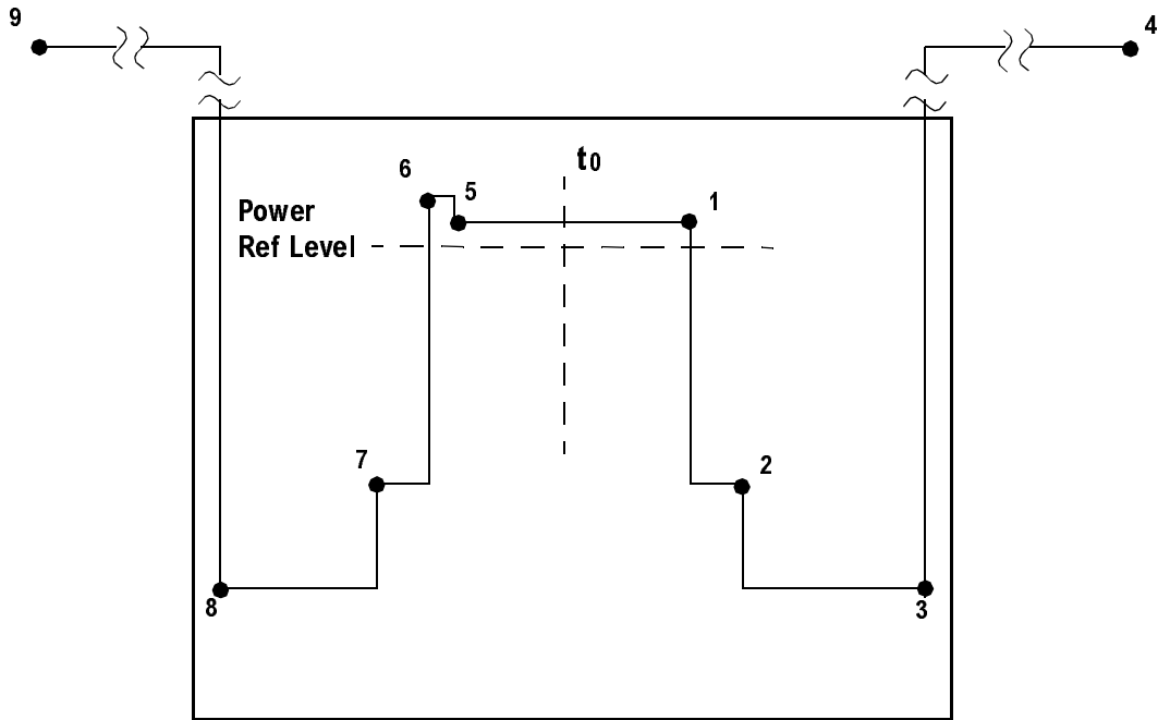
Figure 5-2 Custom Upper Limit Mask Example
