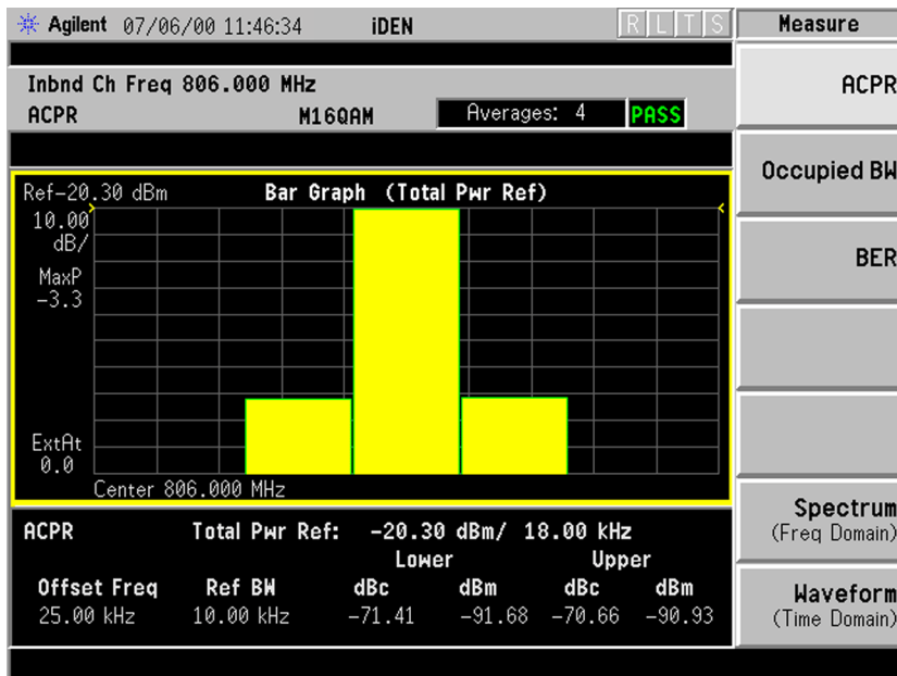
Figure 3-1 Adjacent Channel Power Measurement Result - Bar Graph
