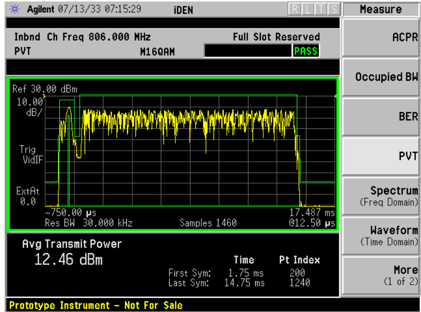
Figure 3-4 iDEN Power vs. Time Result - Burst View
