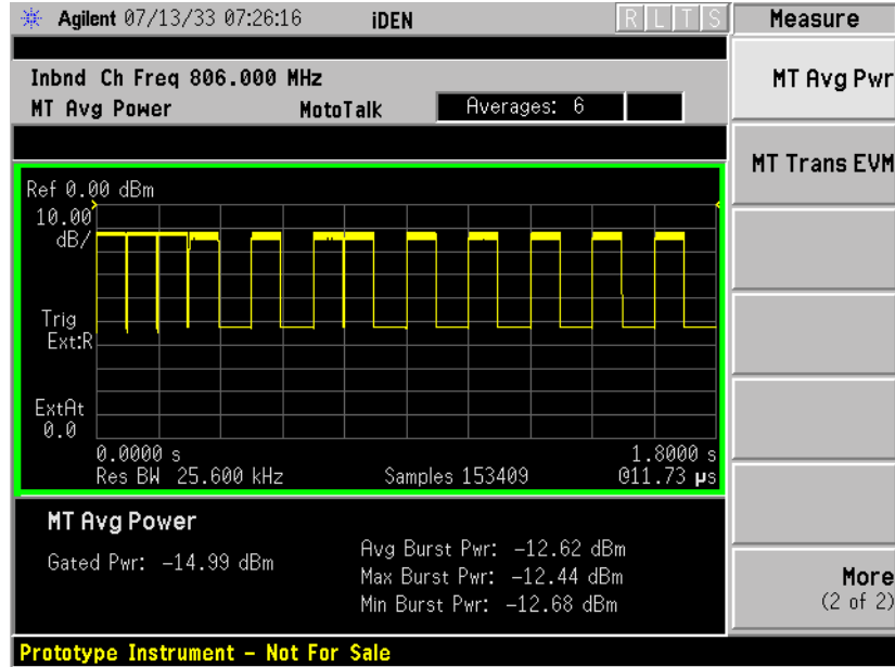
Figure 3-6 Average Power Measurement Results- RF Envelope Window
