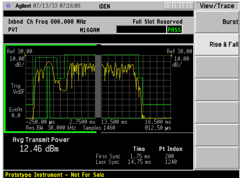
Figure 3-5 iDEN Power vs. Time Result - Rise & Fall View
